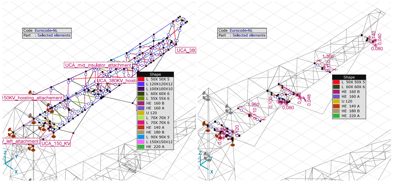
Upper_cross_arms_details
