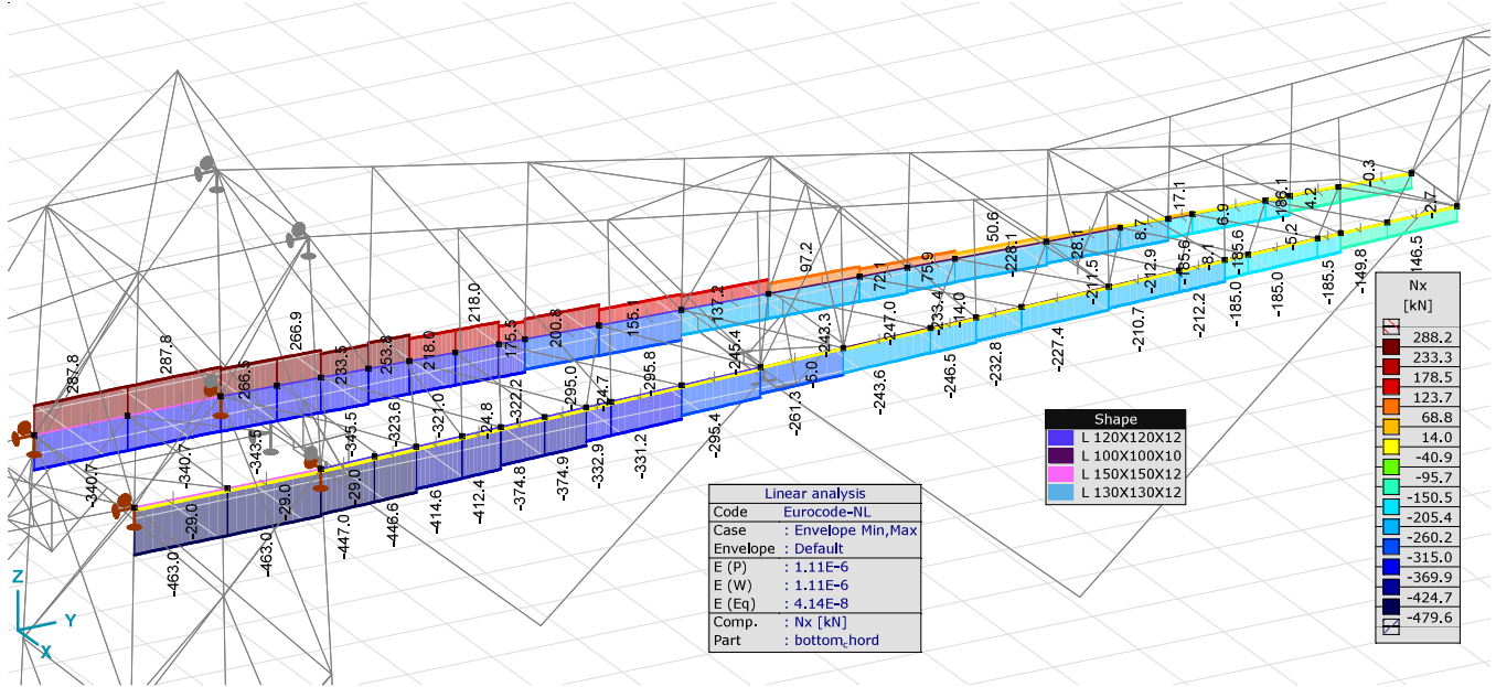
UCA_bottom_chord, Linear, Envelope (Default), Nx [kN], Filled diagram
