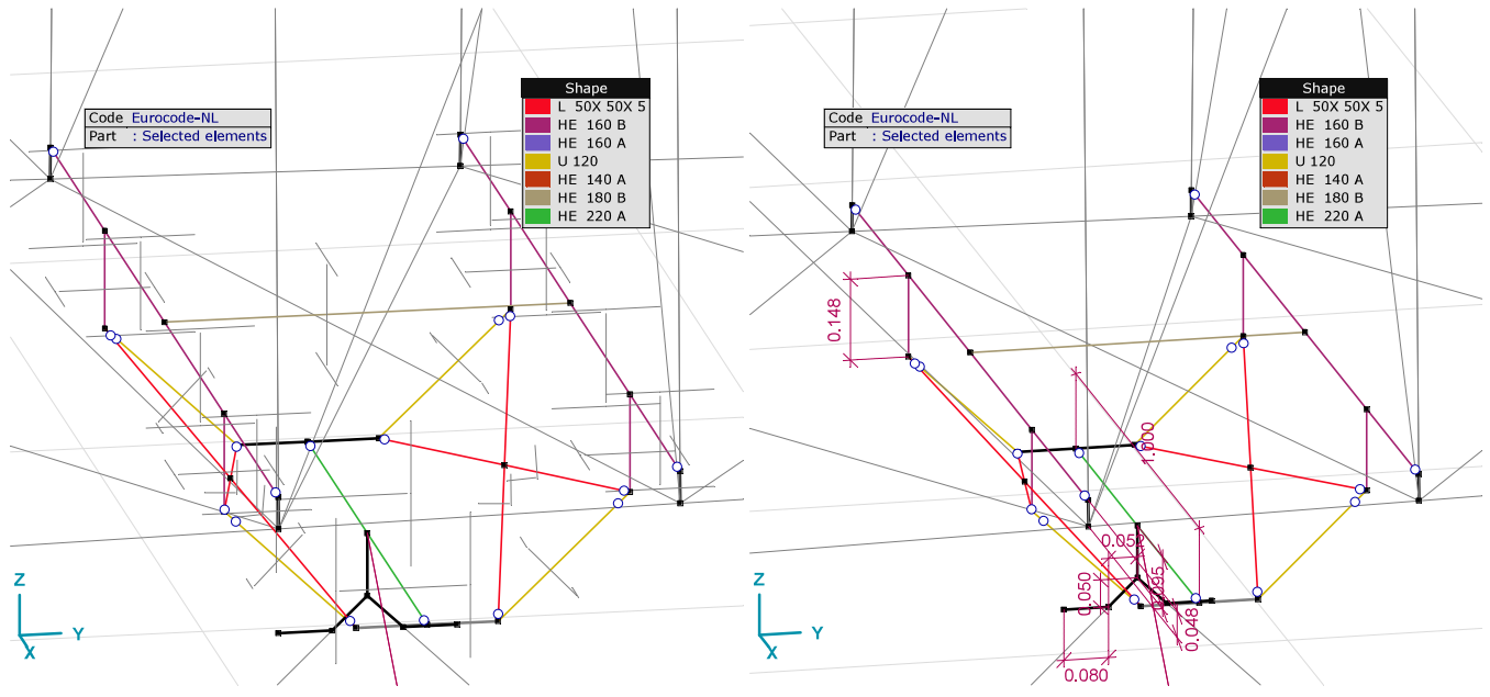
MCA_mid_attachment_(1)_cross-section_orientation_(2)_dimension
