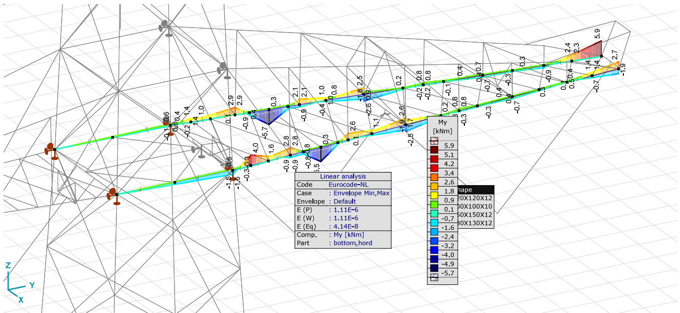
LCA_bottom_chord, Linear, Envelope (Default), My [kNm], Filled diagram
