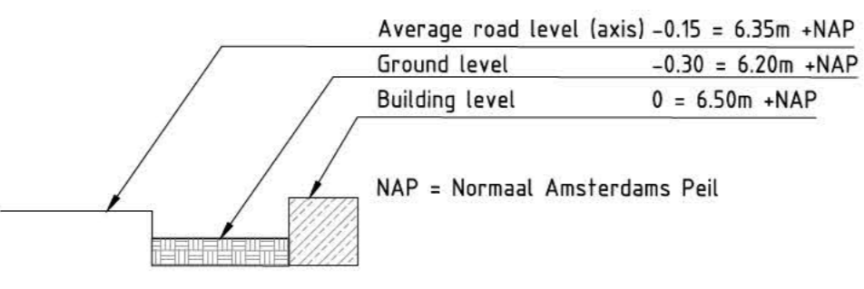
Principe detail bouwpeilen aanlegssituatie Beta & Gamma / Principle detail construction situation levels Beta & Gamma Schaal 150 / Scale 150
