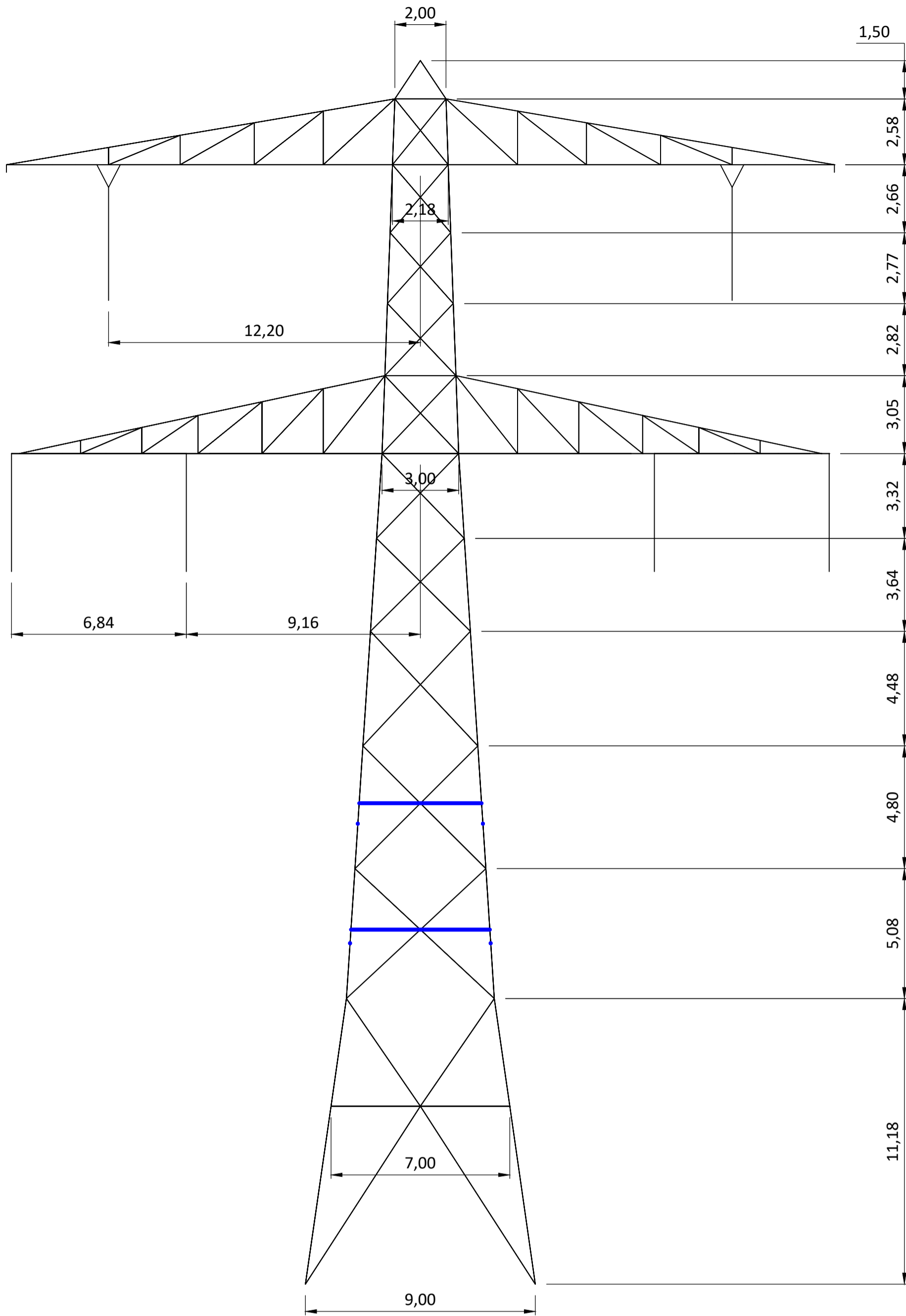
Front View
