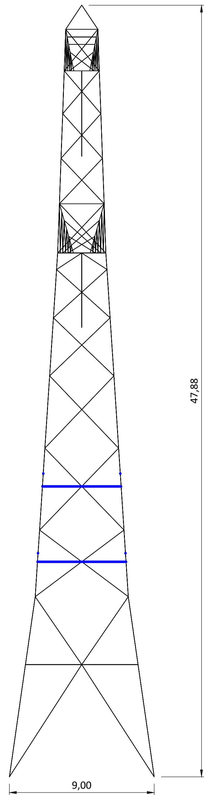
Side View
