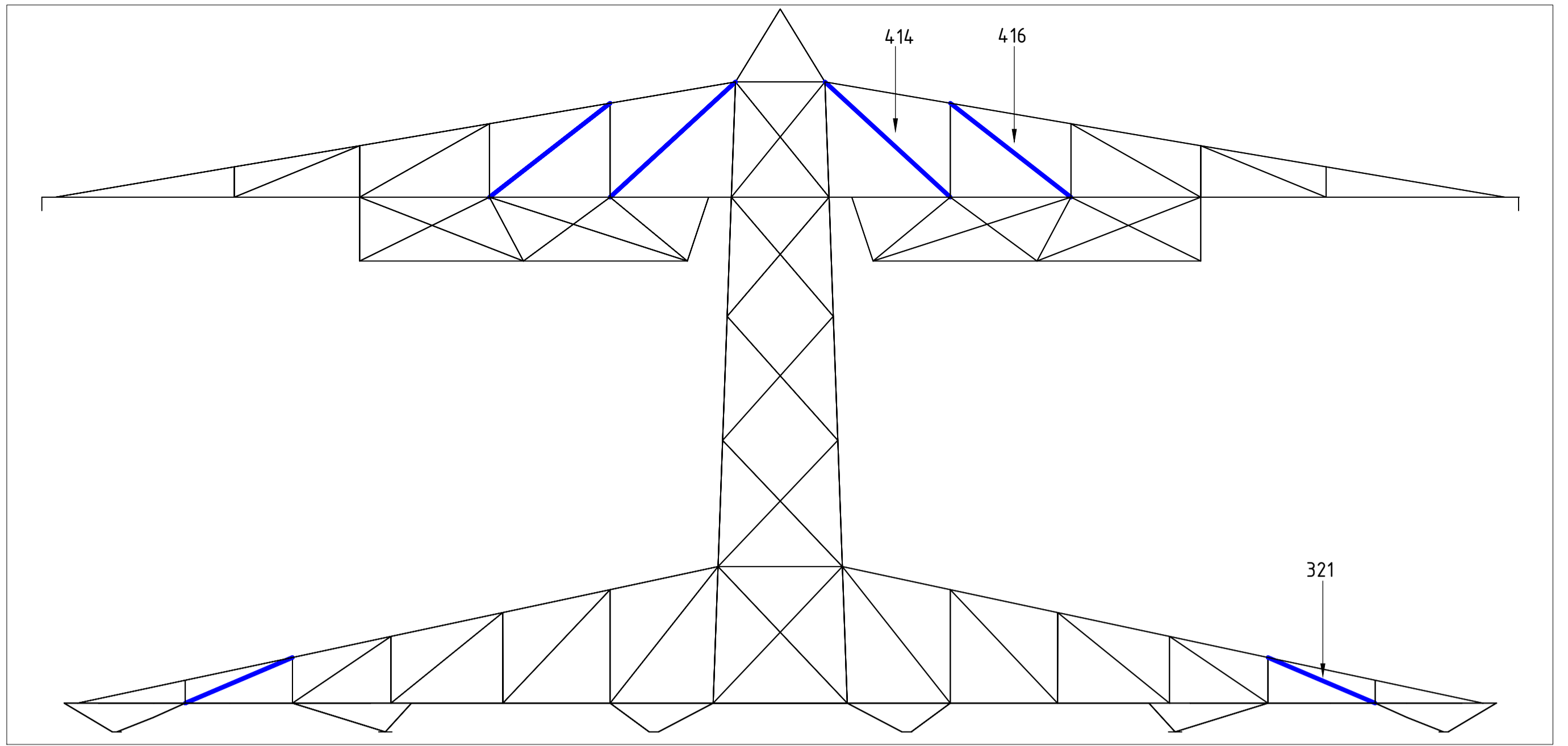
Front View Crossarms
