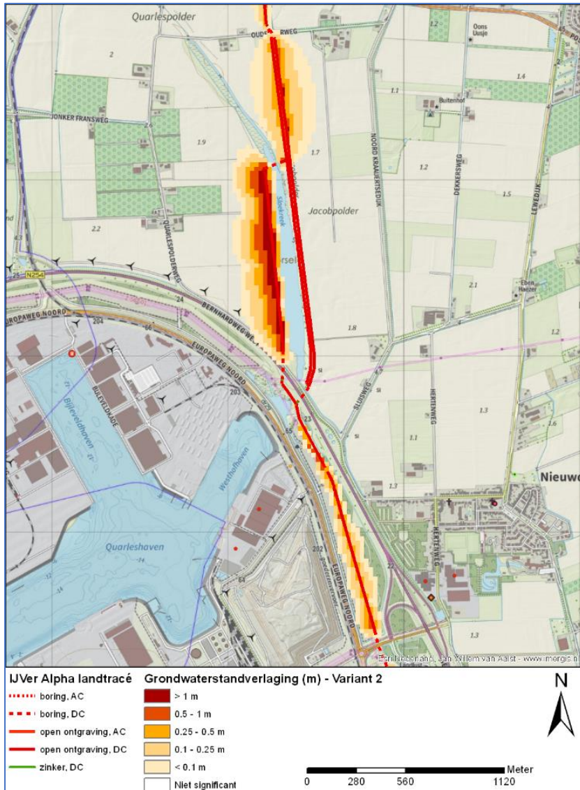
Figur 5-5 Grondwaterstandverandering VKA-tracé - variant Sloekreek West
