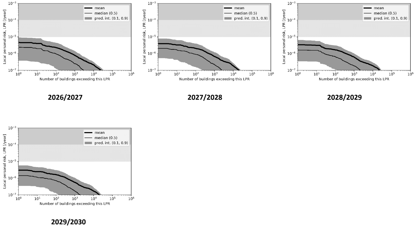
Figure 7.1b Local Personal Risk graphs for the gas-years 2026/2027 to 2029/2030. These show the number of houses exceeding a certain LPR. The thick black lines denote the mean and the dark grey areas the uncertainty bands. The two horizontal bands in light grey denote the LPR levels of the Meijdam-norm. The assessment is based on production profile “GTS-raming 2019” for an average temperature year and Operational Strategy 1.
