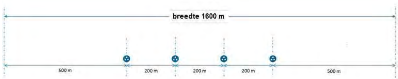
Figure 33 Cable corridor offshore section - 4 cable systems
